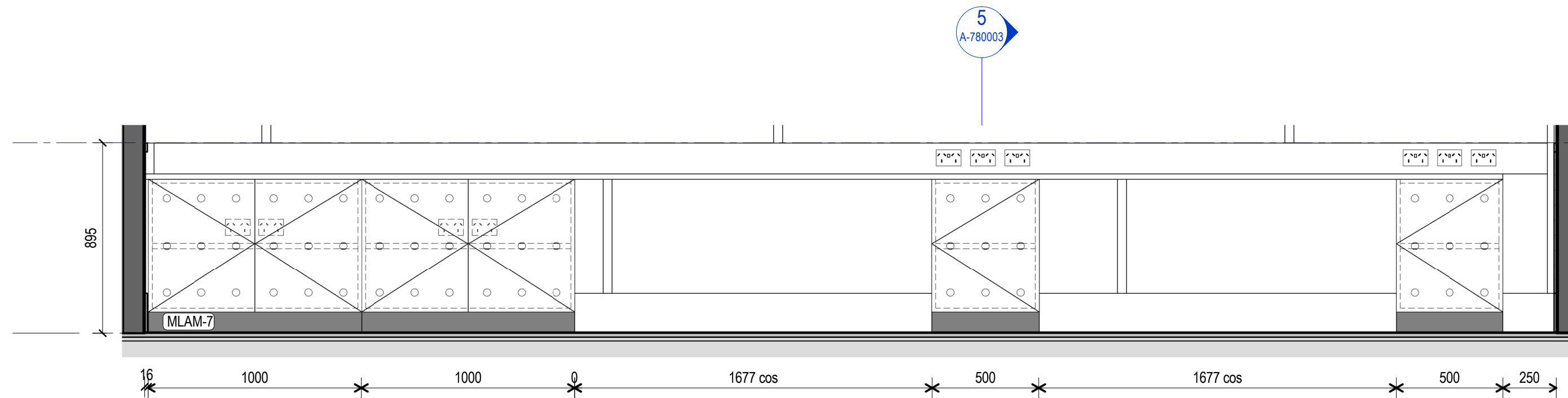
36 JO-BD-5a - Elevation 1 : 20
