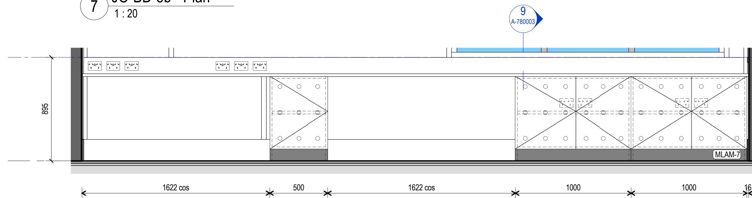
8 JO-BD-5b - Elevation 1 : 20
